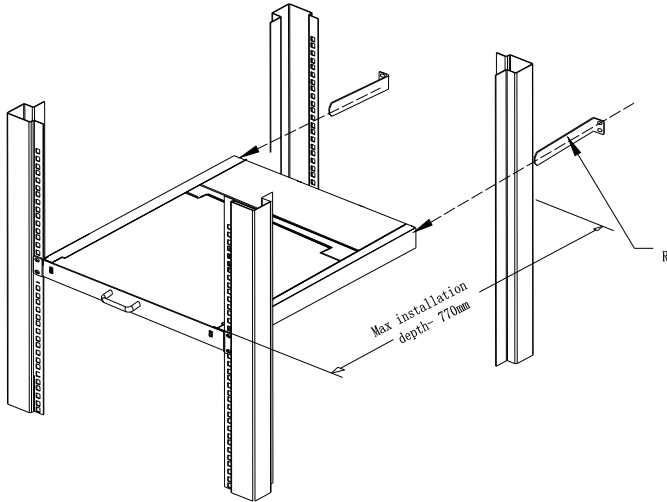
2-1.1 rack mounting (1)
