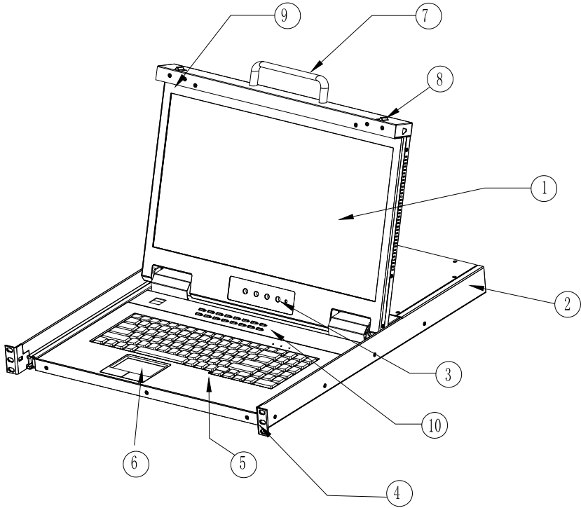
1-1.1 front view
