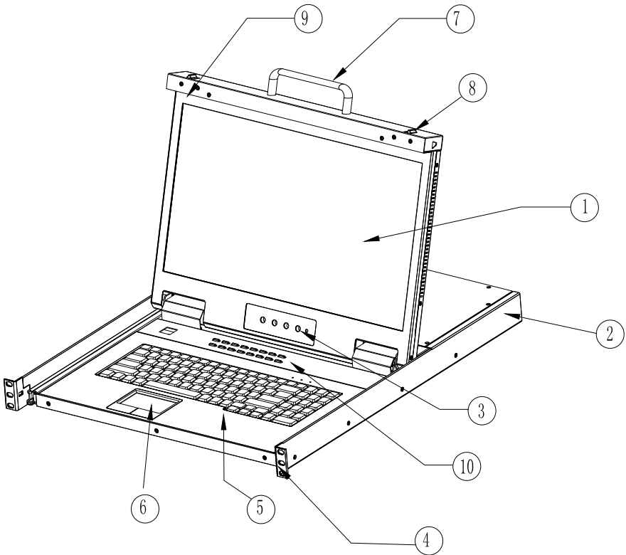
1-1.1 front view
