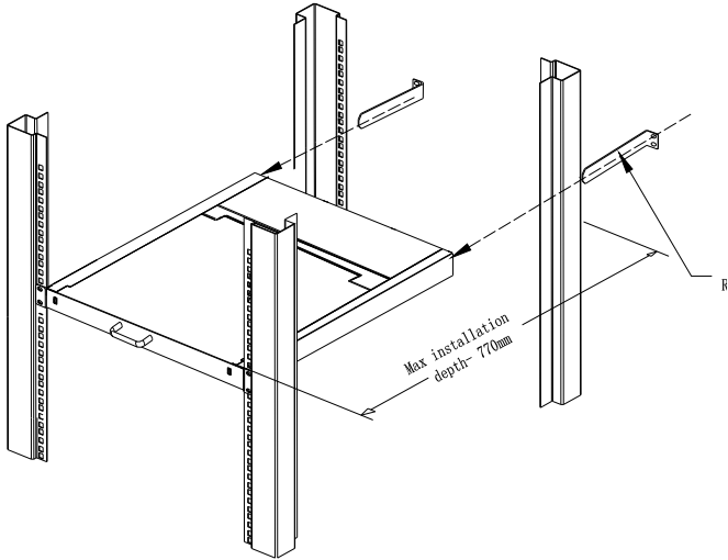
2-1.1 rack mounting (1)
