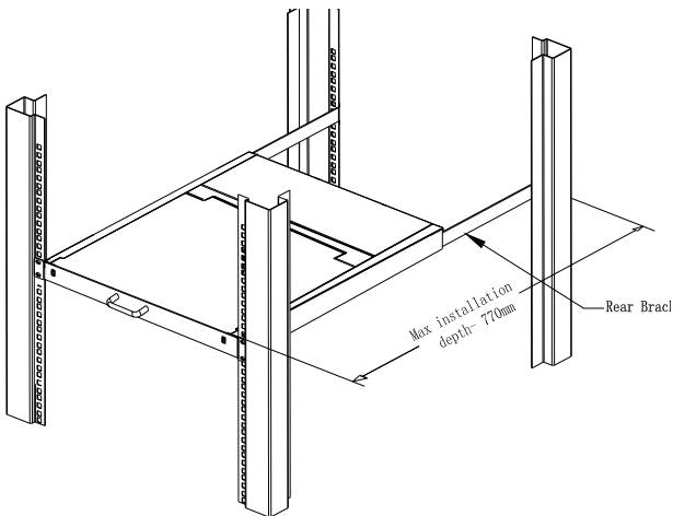
2-1.2 rack mounting (2)
