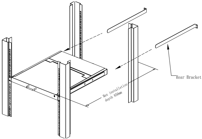
2-1.1 rack mounting (1)
