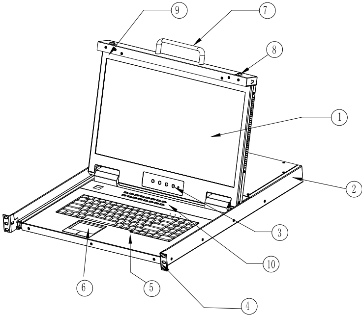
1-1.1 front view
