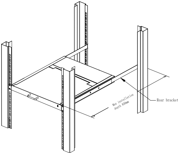
2-1.2 rack mounting (2)
