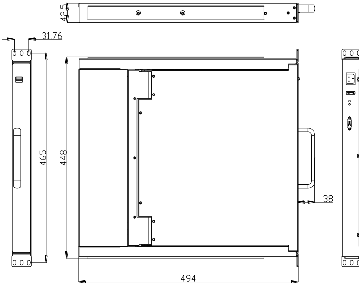
1.1 appearance
