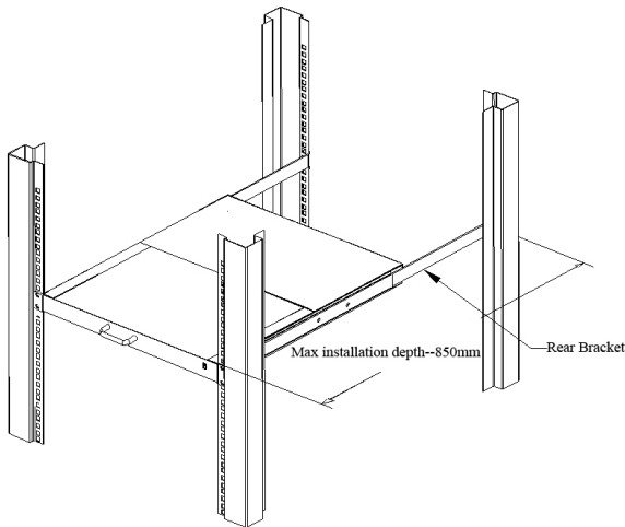
1-2.2 rack mounting (2)
