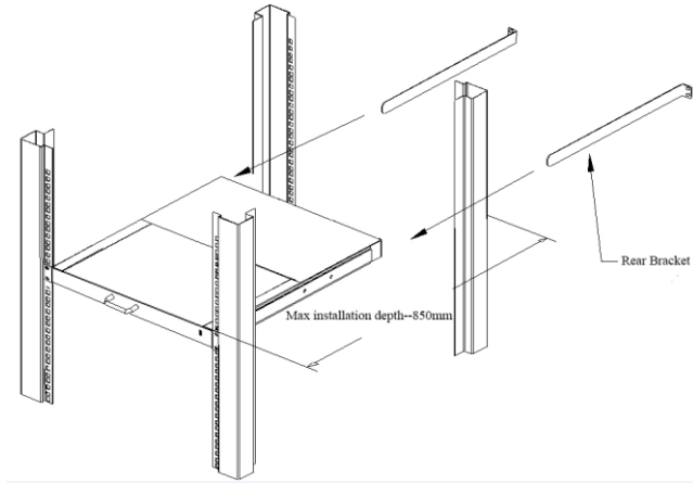
1-2.1 rack mounting (1)
