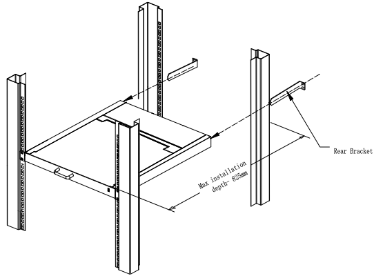
Figure 2-1.1 rack mounting (1)
