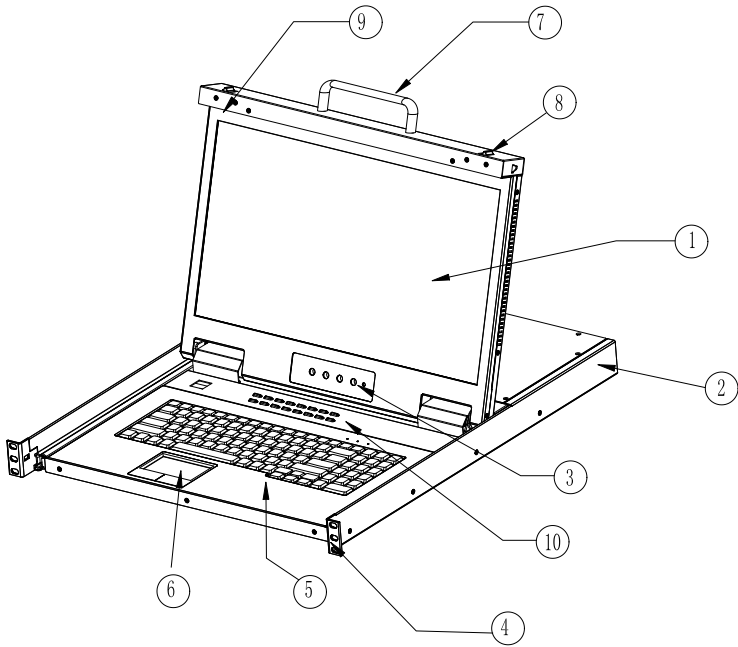
1-1.1 front view
