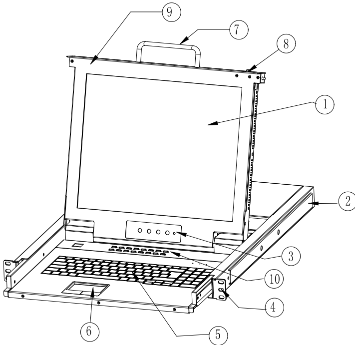
Figure 1.1 Front view
