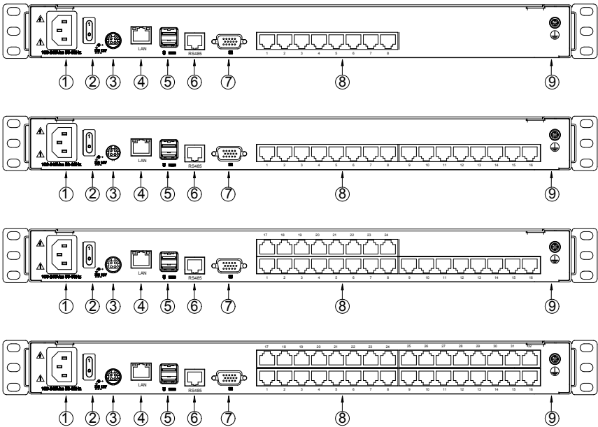
Figure 1.2 Rear view
