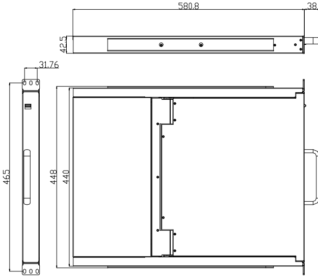
Figure 1.3 17" console size dimensions
