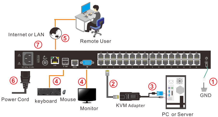
2-2.1 Installation diagram
